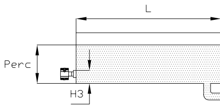
Cylindrical horizontal tank
