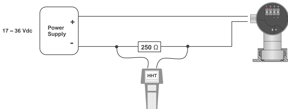
Option 2: HART® Handheld terminal connected across the loop resistor.
