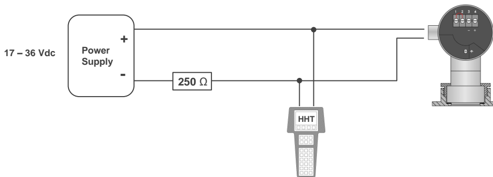
Option 1: HART® Handheld terminal connected across the transmitter.
